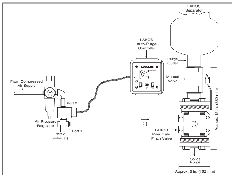
SUGGESTED INSTALLATION
